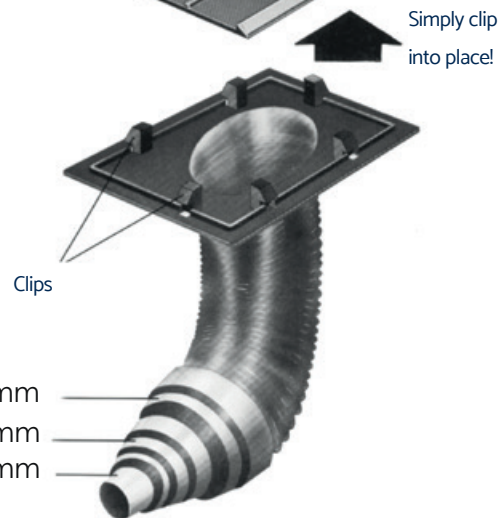
Outlet vent connection
